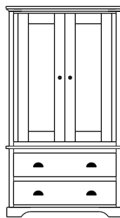
2 adj shelves & 1 pole 37x19x66 31-3552- __ 25" Deep: 31-3592-__ Wardrobe: 31-3582-__
