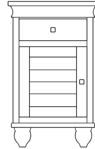
1 adj shelf 21x19x34 37-4981-__
