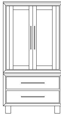
2 adj shelves & 1 pole 37x19x67 31-6652 -__ 25" Deep: 31-6692-__ Wardrobe: 31-6682-__
