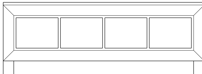
Queen-Size Footboard (24" high)
